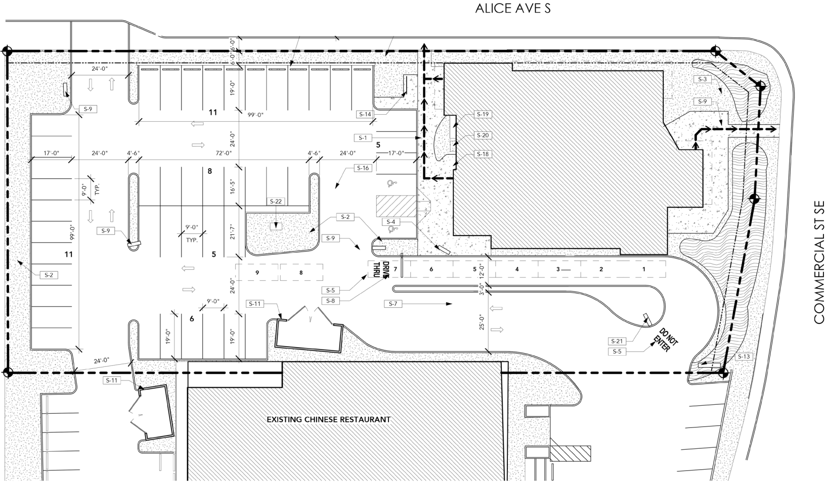
1 SITE PLAN 1" = 20'-0"
