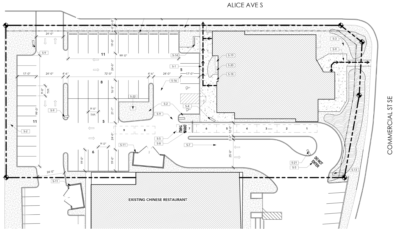
1 SITE PLAN 1" = 20'-0"
