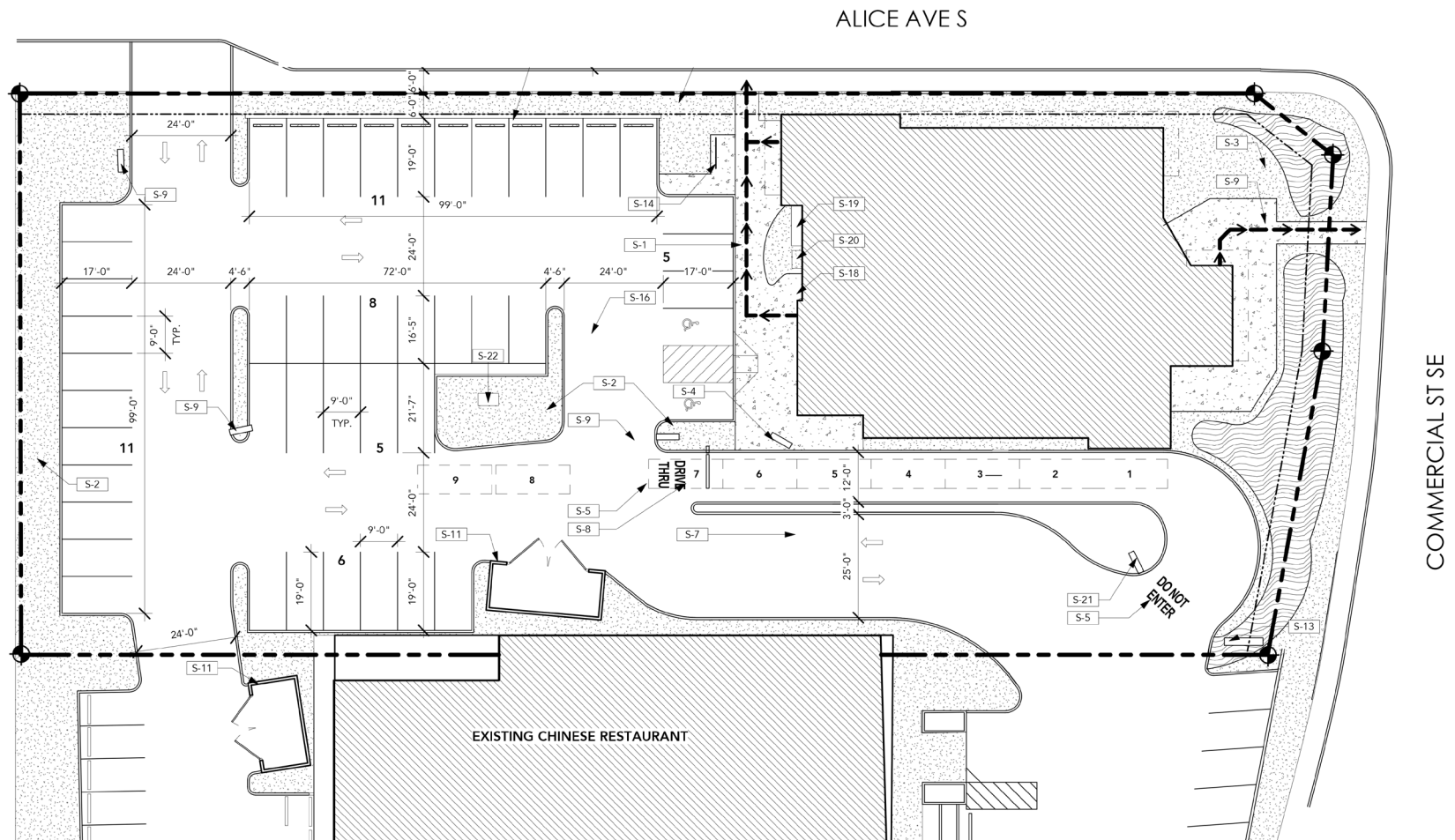
1 SITE PLAN 1" = 20'-0"
