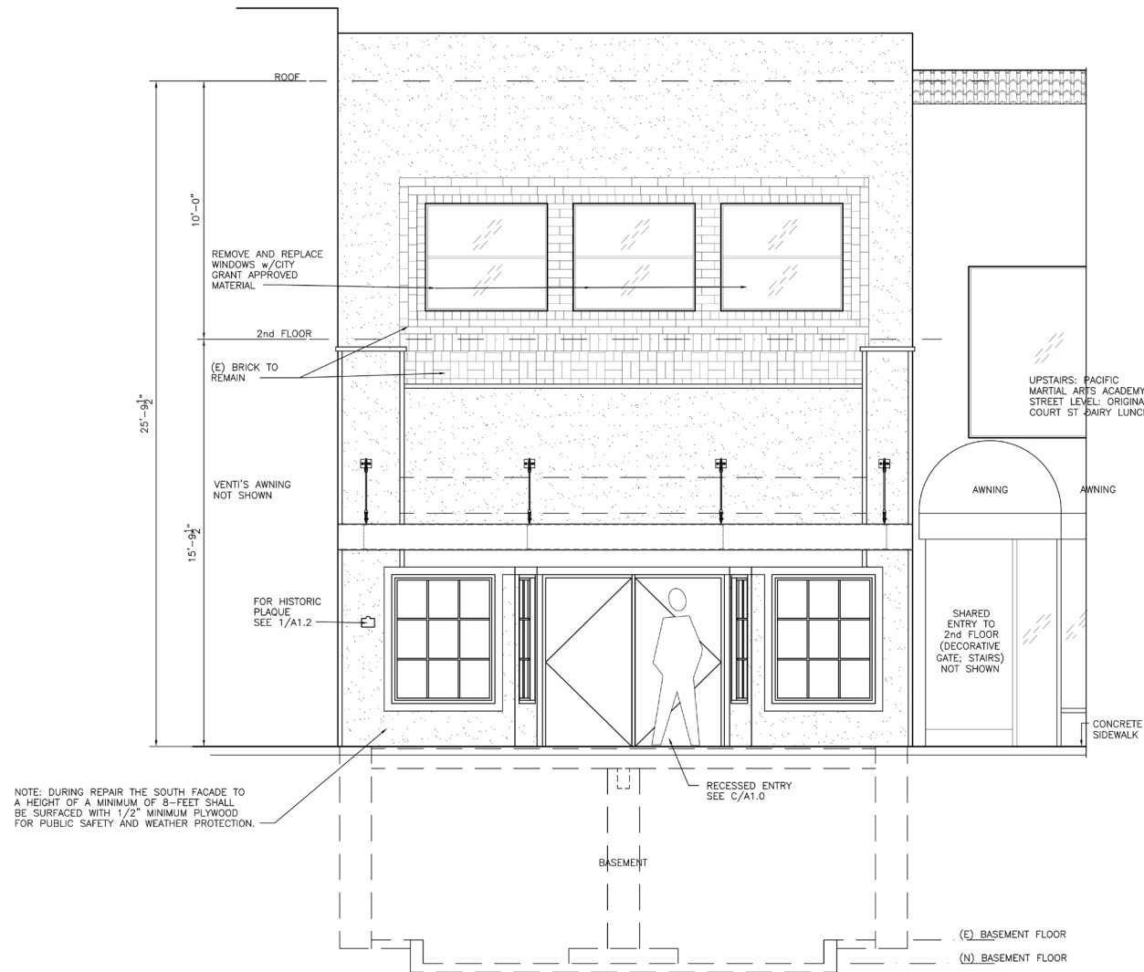
A FACADE REPAIR / SOUTH ELEVATION
