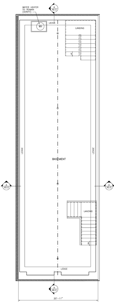
A BASEMENT PLAN SCALE: 1/4"=1'-0" N
