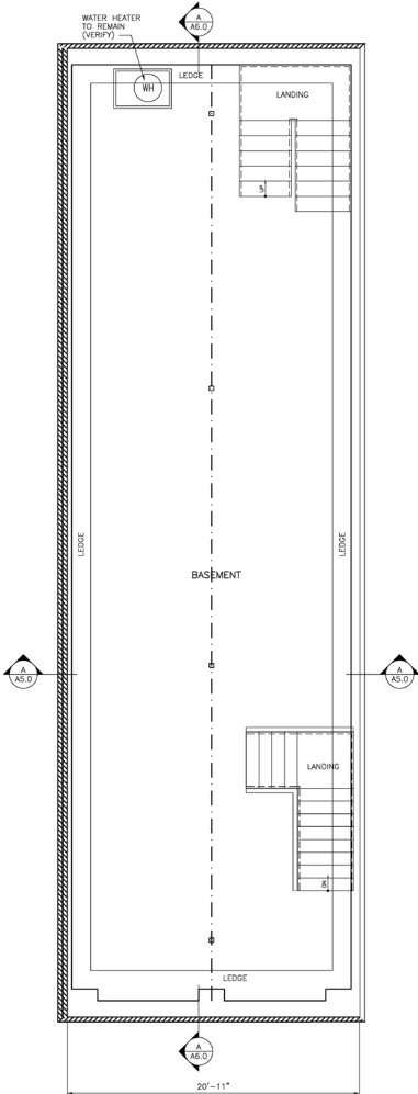
A BASEMENT PLAN SCALE: 1/4"=1'-0"
